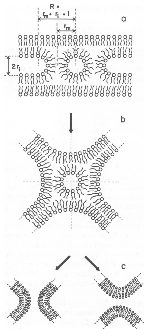
FIGURE 2 (a) IMI structure in cross section. The inverted micelle is spherical. The structure is cylindrically symmetrical about the vertical axis (dashed line through the center of the micelle). (b) Rearrangement of the bilayer attachments to the IMI. The structure is still cylindrically symmetrical about the vertical axis. (c) Products of IMI reversion to bilayer structures. Left : fusion of the two original lamellae, resulting from rearrangement of the micellar lipid around the vertical axis of b . Right : re-formation of original lamellae, resulting from rearrangement about the horizontal plane of symmetry (dashed horizontal line in b ).
