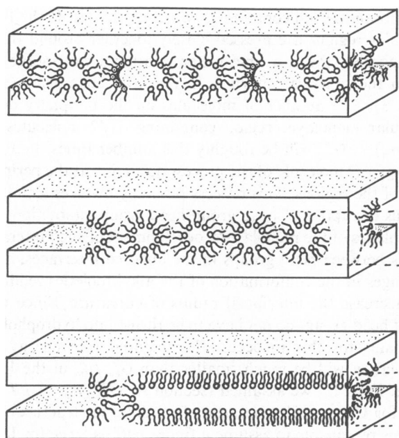
FIGURE 4 IMI aggregation into H_{II} rod precursors. Top : many IMI form between apposed lamellae. Middle : IMI encounter others and aggregate forming strings of inverted micelles enveloped by the lipid monolayers of the apposed lamellae. Bottom : micelles aggregate into elongated cylindrical micelles ( H_{II} rod precursors). Only the lipid molecules composing the IMI and the H_{II} rod precursors are depicted.
